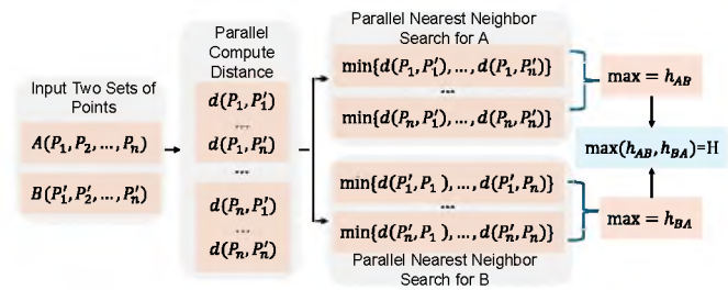
Fig. 8: The 3D similarity calculation provides efficient similarity analysis to identify points to be filtered out.
