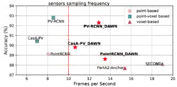
Fig. 2: Detection speed of different methods. The point-based and point-voxel based detection networks process fewer than 10 frames per second. The voxel-based detection networks are faster but have a larger accuracy loss.
